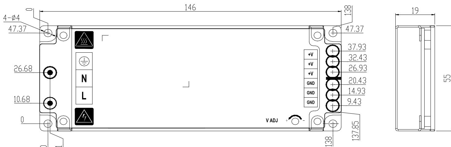
Dimensions and mounting holes - terminal coordinates
